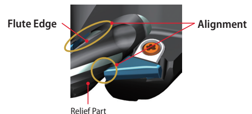
Fig.4 DRA Alignment
